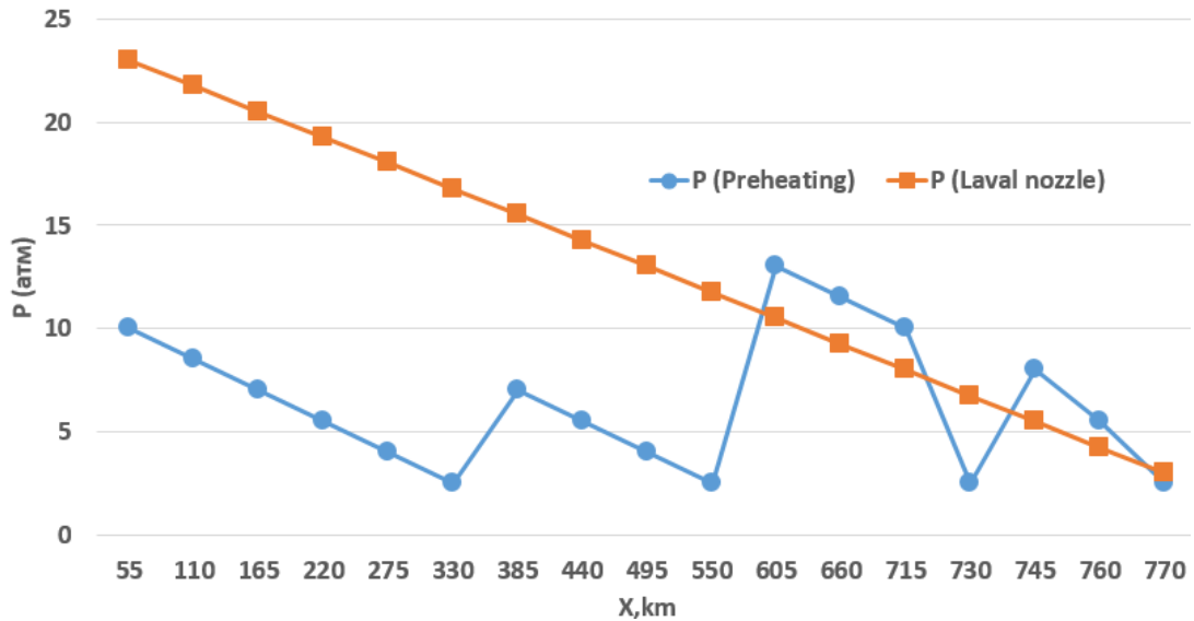
Figure 1 - Pressure distribution along the Uzen-Atyrau oil pipeline
