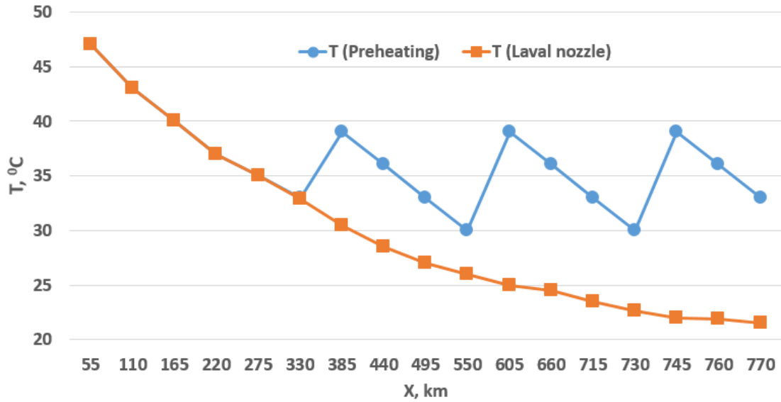
Figure 2 - Temperature distribution along the Uzen-Atyrau oil pipeline
