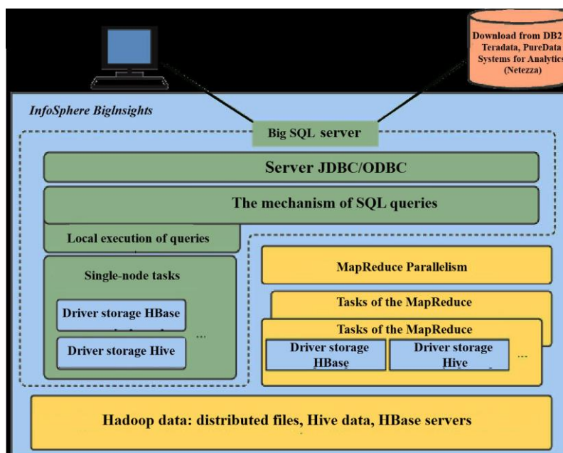
Figure 1. BigSQL architecture.
