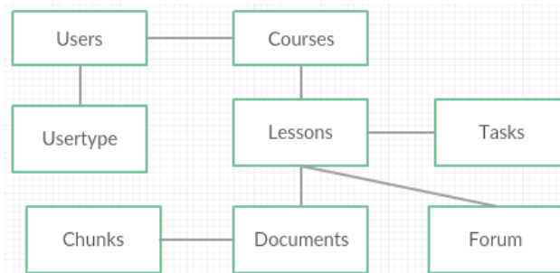
Figure 4 – Database entities
