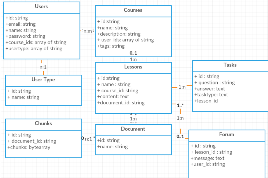
Figure 5 – Database structure
