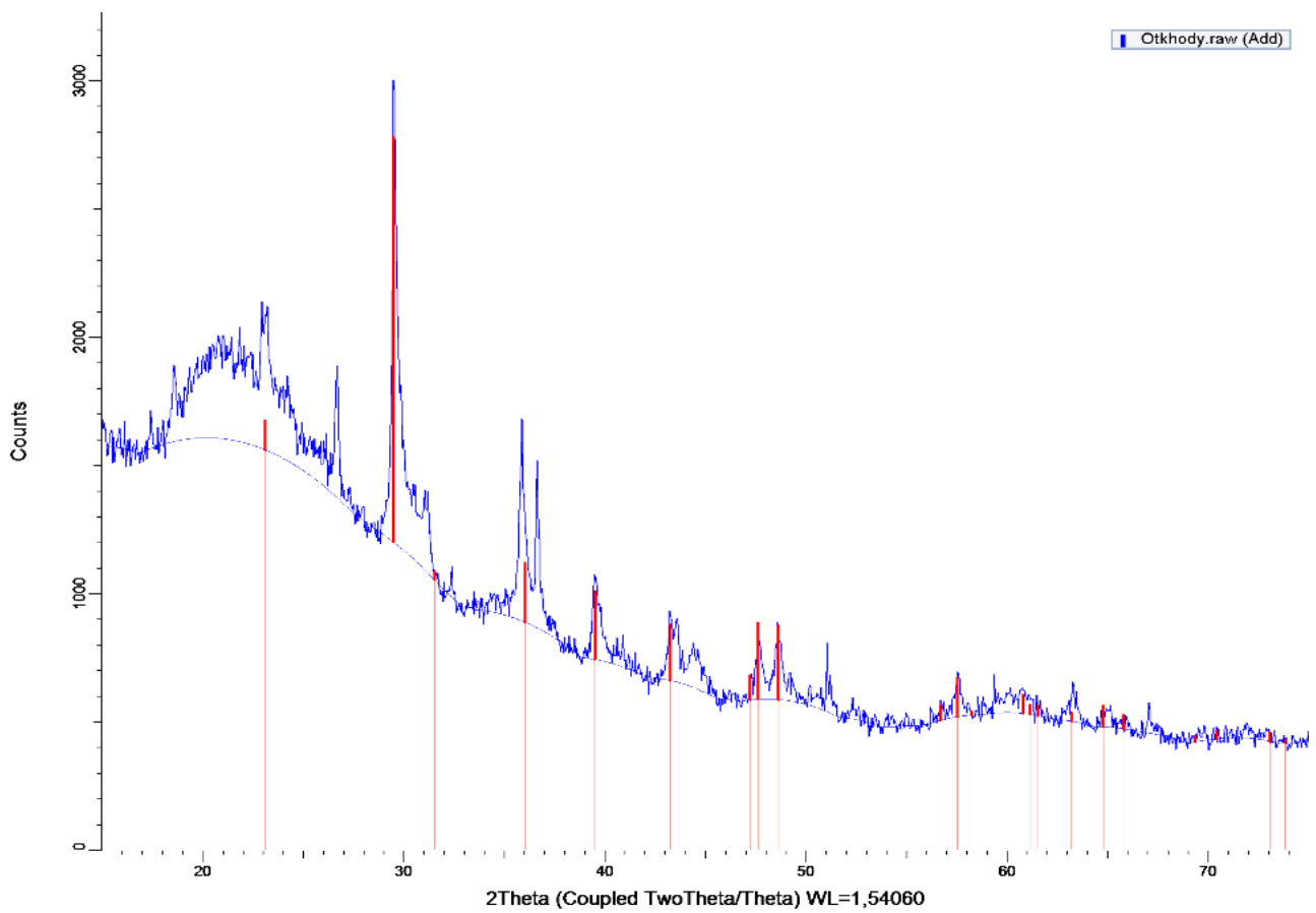
Fig. 3 – Diffractogram of the sample of the WFP.
