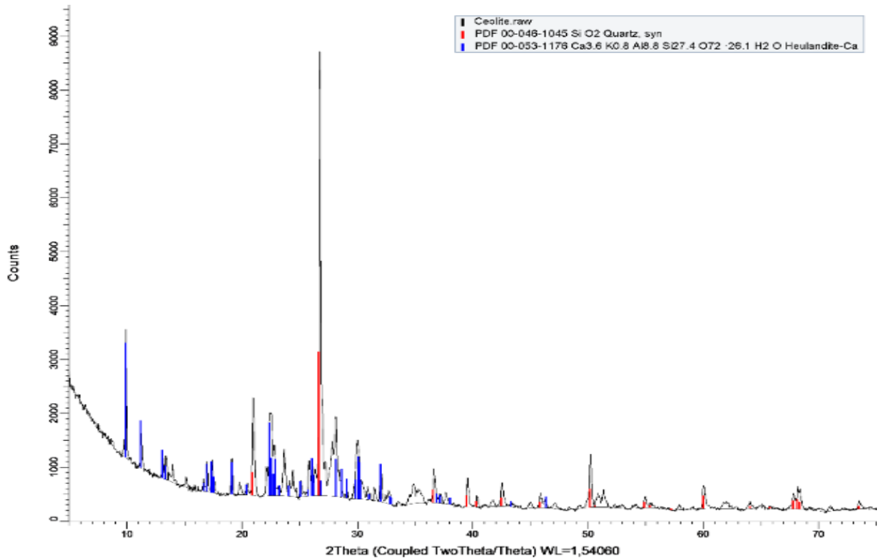
Fig. 2 – Diffractogram of a sample of zeolite with the detection of heulandite and quartz.
